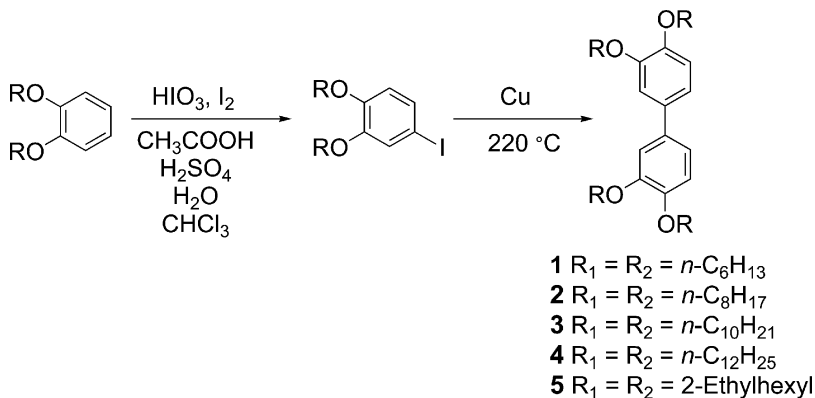
SCHEME 1 Synthesis of 3,3',4,4'-tetrakis(n-alkoxy)biphenyls.
