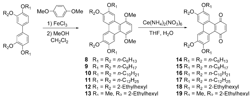
SCHEME 3 Synthesis of mesogenic triphenylene quinones.
