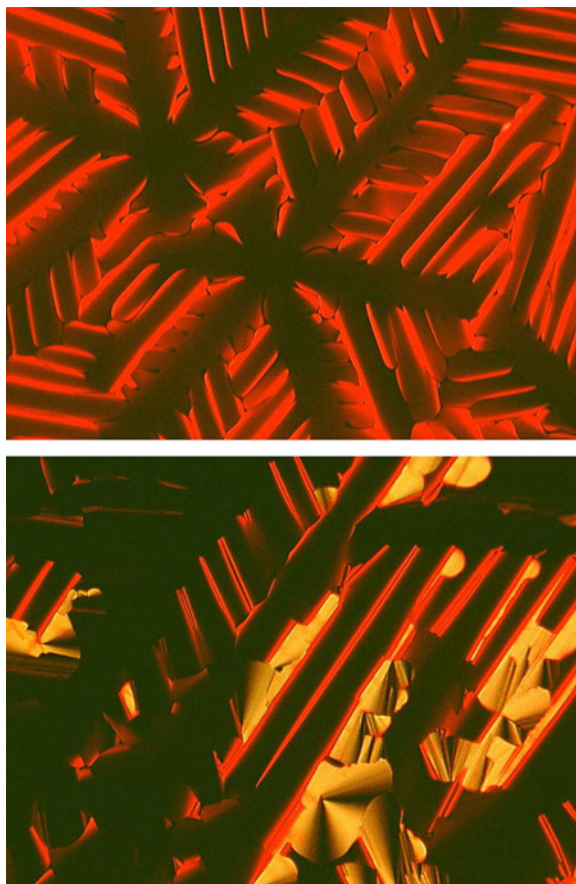
FIGURE 1 Polarized microscopy of the Col h phase of 15 at 111°C (top) and 109°C (bottom) (both 100 × magnification). (See COLOR PLATE XI)
